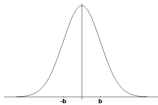
Normal distribution
