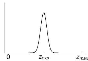
Measurement noise
