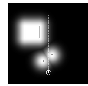
Likelihood field
