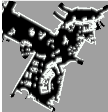
Likelihood field
