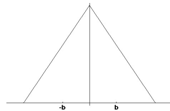
Triangular distribution
