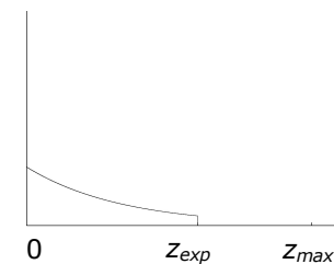
Unexpected obstacles
