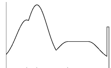
Likelihood field
