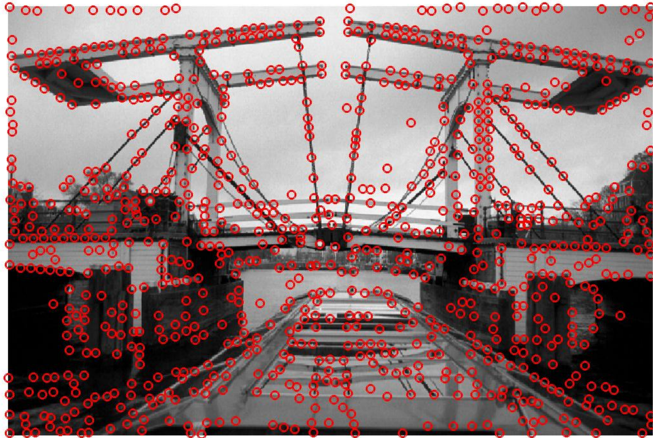
Harris Corners
