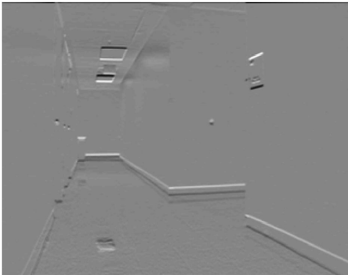
Horizontal edges
