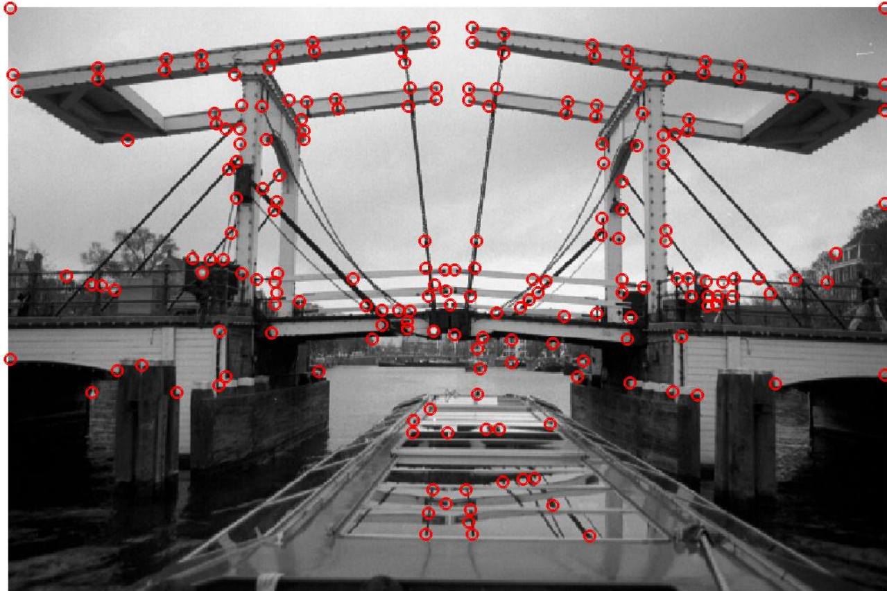
Harris Corners
