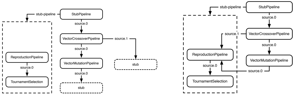
Figure 3.4 Stub Pipeline before (as specified in the parameter file) and after (as constructed). See text.
