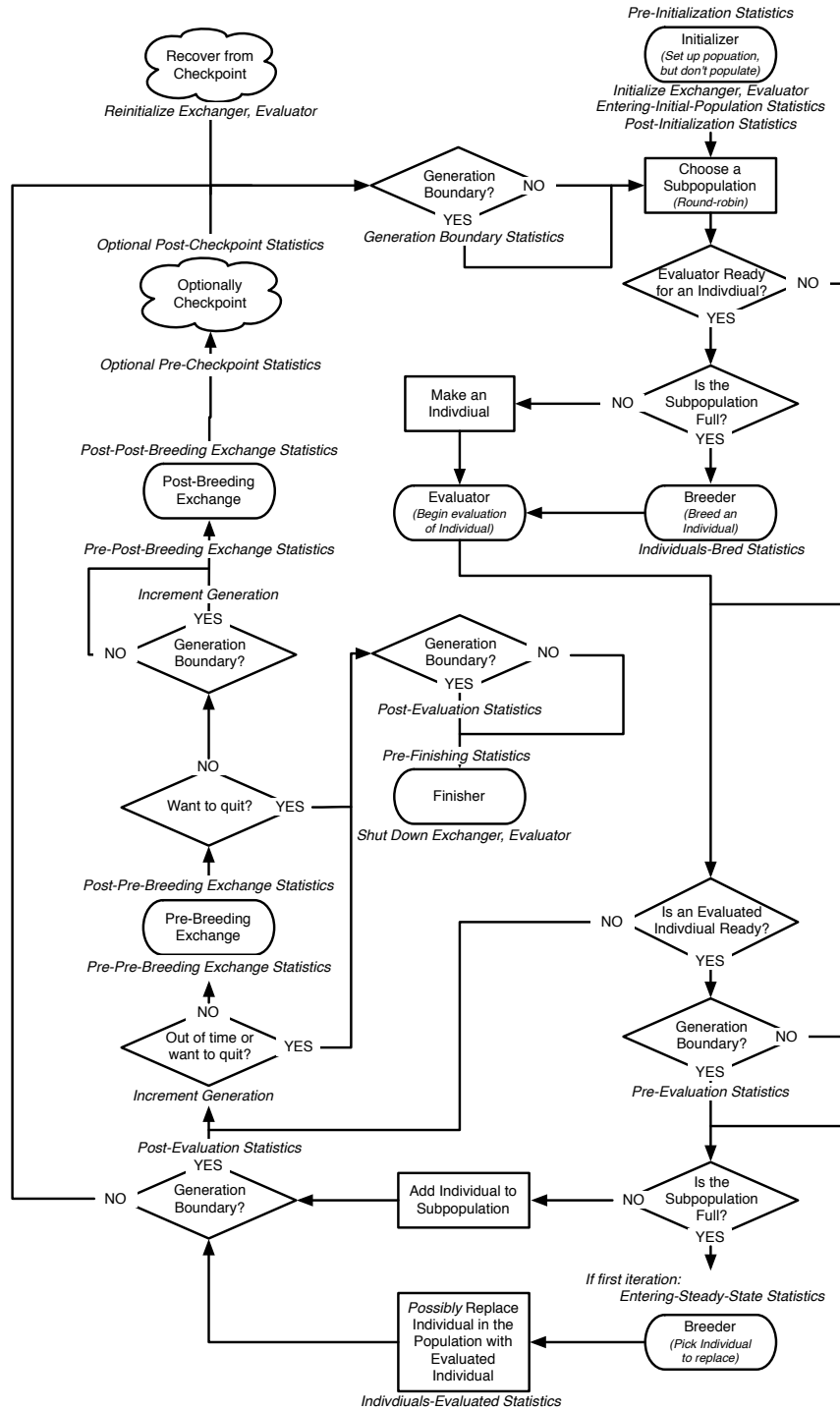
Figure 6.2 Top-Level Loop of ECJ's SteadyStateEvolutionState class, used for simple steady-state EC and Asynchronous Evolution algorithms. "First?" means to perform the Statistics whenever the Subpopulation in question is picking an Individual to displace for the very first time. (Each Subpopulation will do it once, but possibly at different times). A repeat of Figure 4.2.
