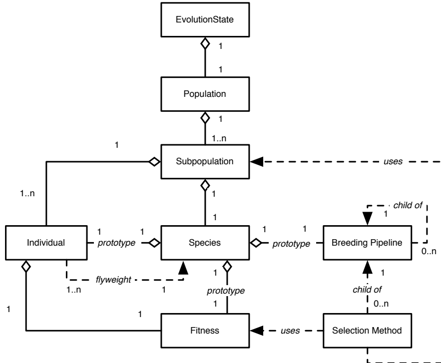
Figure 1.3 Top-Level data objects used in evolution.
