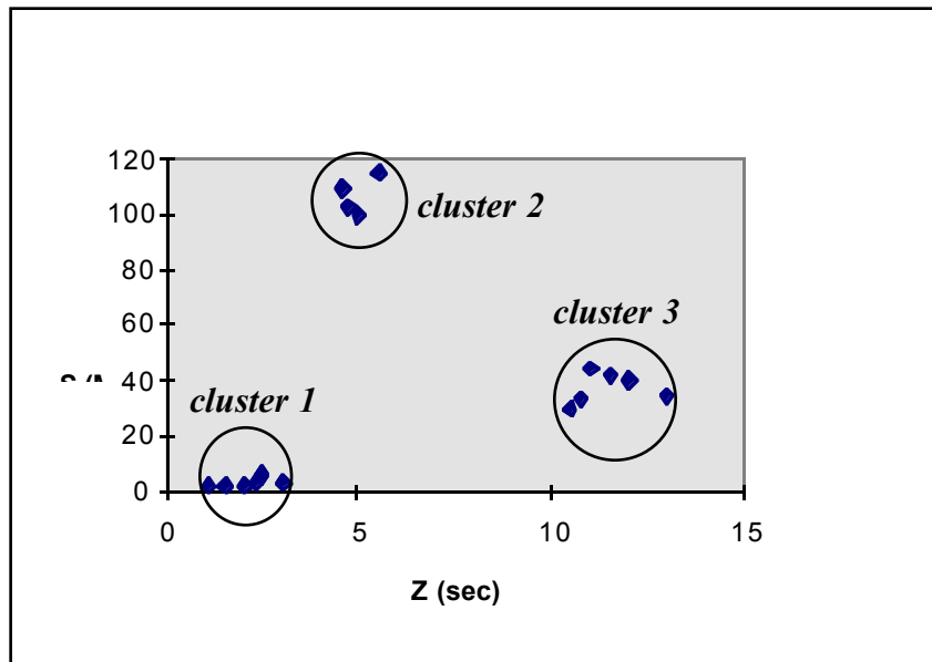
Figure 1 - S versus Z scatter plot.
