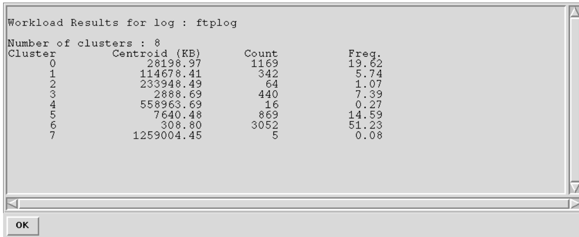
Figure 10 - Workload Window
