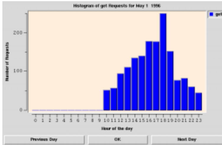
Figure 6 - Histogram Window
