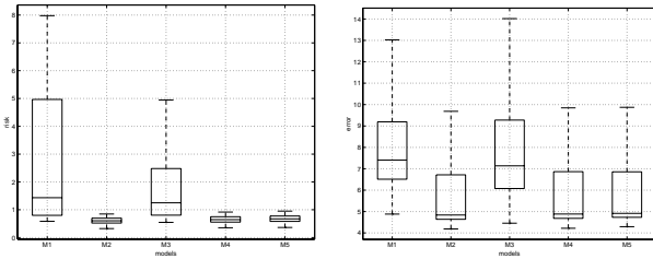
Figure 2. Model selection results for M1, M2, M3, M4 and M5 . Left: boxplots of risks. Right: boxplots of average square errors.
