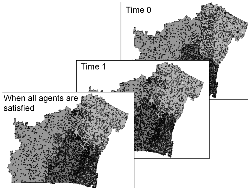
Figure 8. A typical simulation portraying the initial, first, and last iteration until all agents are satisfied when only 5% of the population is white.
