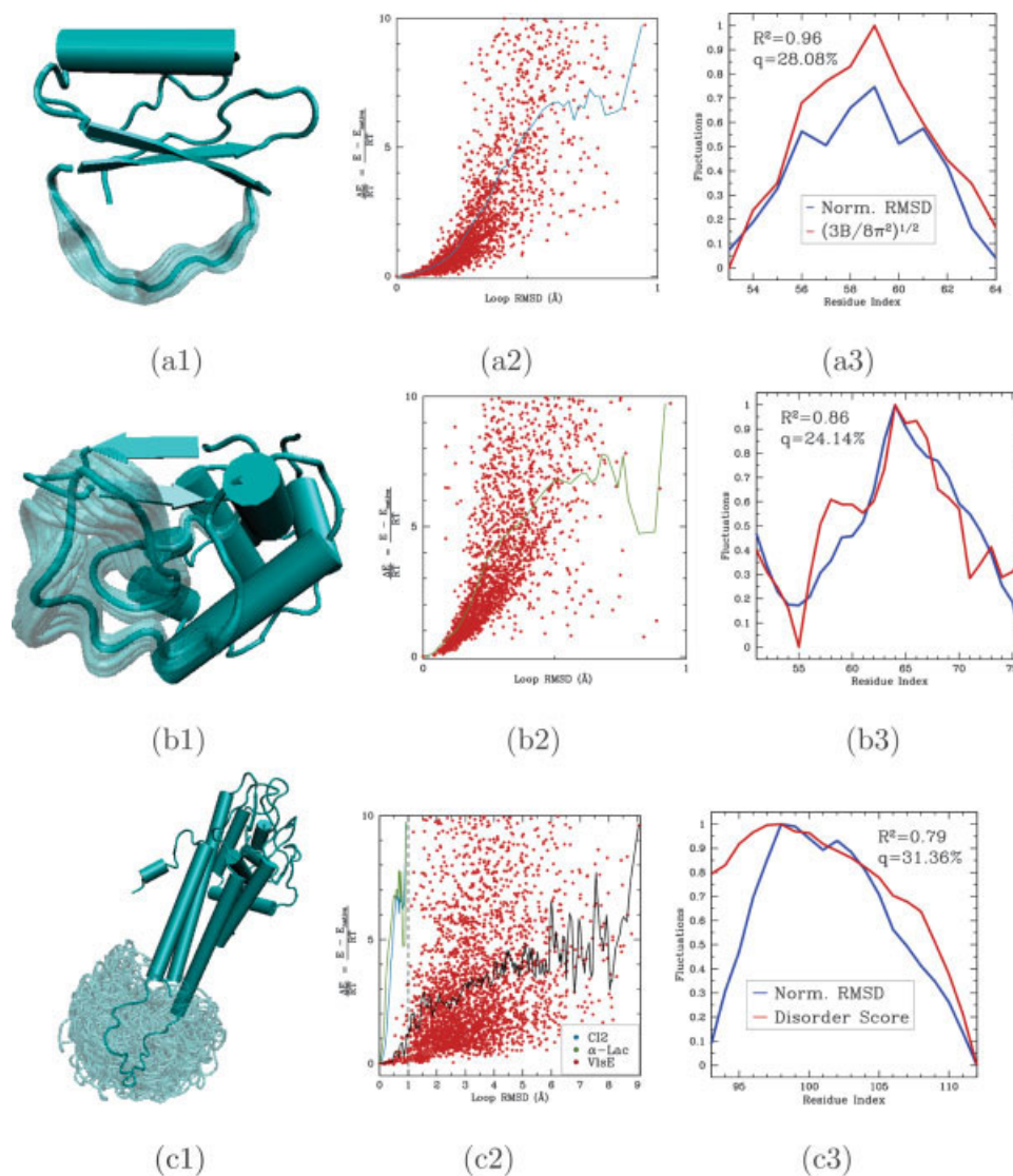
Fig. 2. a1, b1, c1: 5000 transparent loop conformations versus opaque reference structure (equilibrated native structure for CI2 and \alpha -Lac and lowest energy structure for VlsE). Obtained conformations are rendered with the VMD 1.8.3 software. 84 a2, b2, c2: Energy landscapes associated with generated ensembles are shown by plotting the energetic difference versus the RMSD of each conformation relative to a reference structure. Energy landscapes are shown only for conformations with energy less than 10 RT units away from the reference structure (each ensemble is reduced to 2499, 2022, and 2755 conformations). An average energy profile is computed by distributing conformations in bins every 0.001 Å away from the reference structure and measuring the energy of each bin as an average over its conformations. Average energy profiles obtained for CI2 and \alpha -Lac are very steep compared to the flat average energy profile of VlsE. a3, b3, c3: Obtained fluctuations versus B factor-derived fluctuations for the CI2 loop, fluctuations in Vendruscolo et al. 57 for the \alpha -Lac loop, and disorder scores for the VlsE loop.
