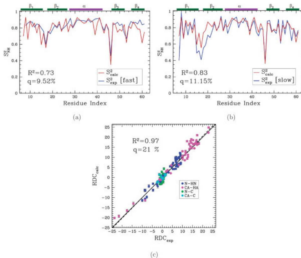
Fig. 4. Comparison of NMR data with thermodynamics data measured over the generated ensemble for protein G. a: Comparison of S^2 backbone (amide) order parameters measured over our ensemble ( S^2_{calc} ) with fast ( S^2_{NH} ) data obtained from NMR relaxation measurements ( S^2_{exp} ). b: Comparison of S^2 backbone (amide) order parameters measured over our ensemble ( S^2_{calc} ) with slow ( S^2_{NH} ) data obtained from NMR relaxation measurements ( S^2_{exp} ). c: Comparison of residual dipolar coupling (RDC) parameters as obtained in our ensemble ( RDC_{calc} , on the y-axis), and from NMR relaxation measurements ( RDC_{exp} , on the x-axis). Results for different bond types are shown in different colors. (a–c) The dashed black line indicates the linear least squares regression fit on the two sets of data, while the continuous line represents the identity line.
