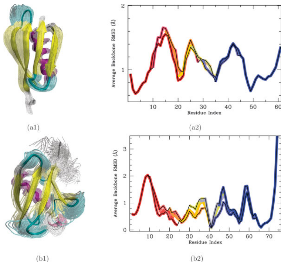
Fig. 3. (a1) and (b1) Obtained native ensembles for protein G and ubiquitin, respectively. (a2) and (b2) Average RMSD per residue obtained by combining the local fluctuations of all the different regions. Results for different regions are shown in different colors, from red to blue as a window of 30 residues slides from the N- to the C- terminus of the protein. The black lines mark the highest and lowest RMSD values recorded from all the different windows embracing each given residue, and provide an estimate for the uncertainty of the procedure. Two consecutive 30-residues windows have an overlap of 25 residues. The results corresponding to the first and last 5 residues of each fragment are discarded as they are biased by the finite size of the window.
