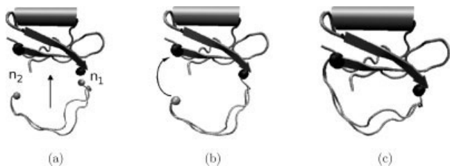
Fig. 1. a: The mobile anchors in two different polypeptide chains for the C12 VAL53-ASP64 loop fragment, drawn in grey, are not attached to the stationary anchors drawn in black. b: Mobile anchor n_1 is attached to its corresponding stationary anchor through rigid body transformations. c: Rotations of the dihedral bonds of the fragment steer the other mobile anchor n_2 towards its target pose in the stationary anchor.
