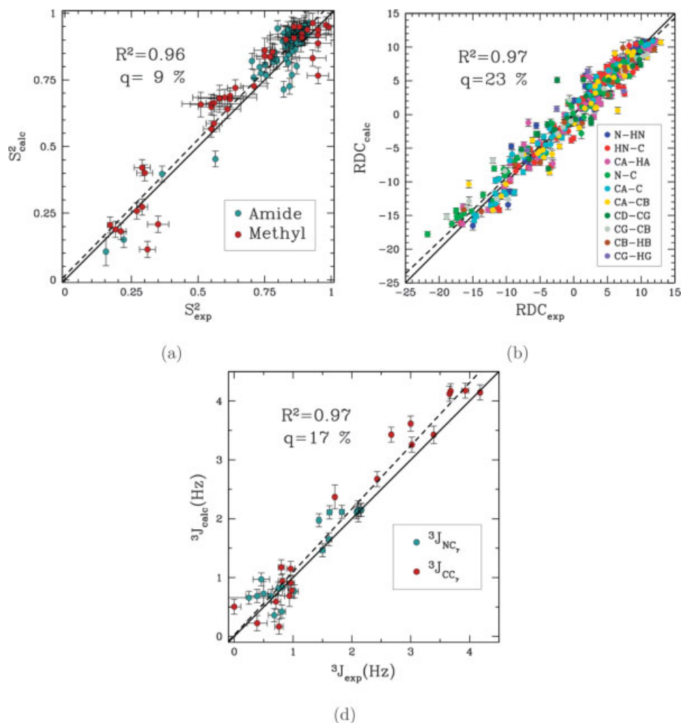
Fig. 5. Comparison of NMR data with thermodynamics data measured over the generated ensemble for ubiquitin. a: Comparison of S^2 order parameters for backbone (amide S^2 ) and side chain (methyl S^2 ), as obtained in our ensemble ( S^2_{calc} on the y-axis), and from NMR relaxation measurements ( RDC_{calc} on the x-axis). b: Comparison of residual dipolar coupling (RDC) parameters as obtained in our ensemble ( RDC_{calc} on the y-axis), and from NMR relaxation measurements ( RDC_{exp} on the x-axis). Results for different bond types are shown in different colors. c: Comparison of three-bond scalar coupling parameters {}^3J_{NC\gamma} and {}^3J_{CC\gamma} as obtained in our ensemble ( {}^3J_{calc} on the y-axis) and as extracted from NMR relaxation experiments ( {}^3J_{exp} on the x-axis). (a–c) The dashed black line indicates the linear least squares regression fit on the two sets of data, while the continuous line represents the identity line.
