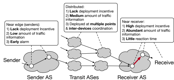
Fig. 6. Information collection for DDoS detection and traffic classification
