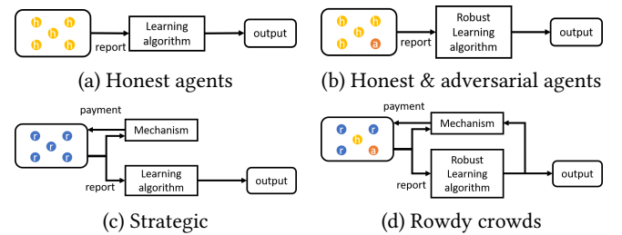
Figure 1: Pipeline models for information elicitation from diverse crowds.
