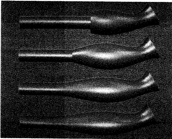
Fig. 12 C^{-1} , C^0 , C^1 and C^2 Local Deformations
