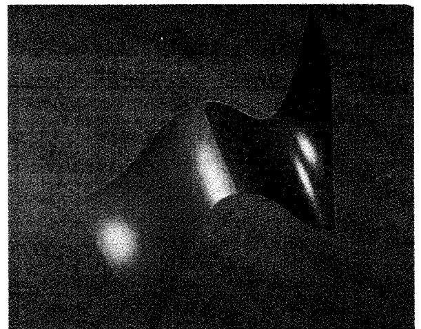
Fig. 17 Two C^1 Bicubic Patches
