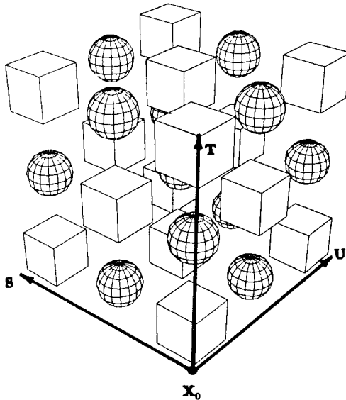
Fig. 3 s, t, u Coordinate System
