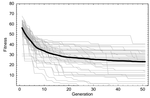
Figure 12: Generation vs. Fitness, UNIFORM-even, Artificial Ant Domain
