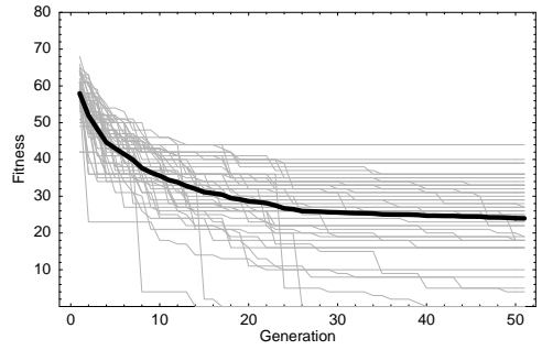
Figure 13: Generation vs. Fitness, UNIFORM-true, Artificial Ant Domain
