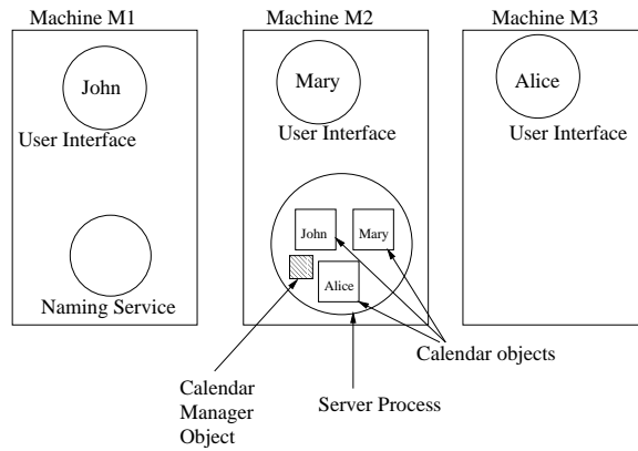
Figure 1: Software architecture for the Calendar tool
