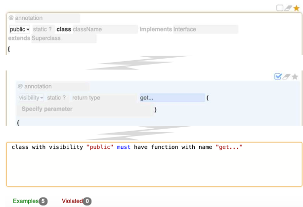
Figure 3: Clicking the golden star on the class updates the Element of Interest to the class. This is reflected in the updated textual description and updated list of violations.
