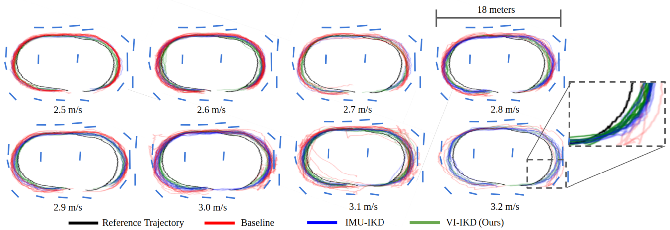
Fig. 5: Trajectory traces for the indoor experiments where the vehicle tracks a reference trajectory counter-clockwise at different speeds. The inset shows Turn 1 as executed by the vehicle at 3.2\text{m/s} using the three approaches. We see that VI-IKD is able to track the reference trajectory more accurately than IMU-IKD [6], confirming our hypothesis. Blue lines along the track show the virtual fixtures used as a map for vehicle state-estimation using EnML [34].
