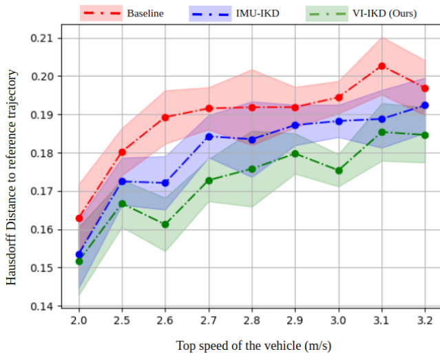
Fig. 6: Hausdorff distance (lower is better) between the reference trajectory and trajectories traced by different algorithms at different top speeds of the vehicle in the indoor evaluation environment. We see that VI-IKD is the most accurate compared to the receding horizon controller with no IKD model (baseline) and IMU-IKD [6].
