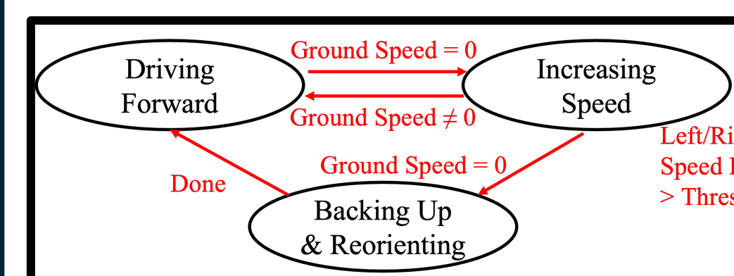
Rule-Based, Open-loop
