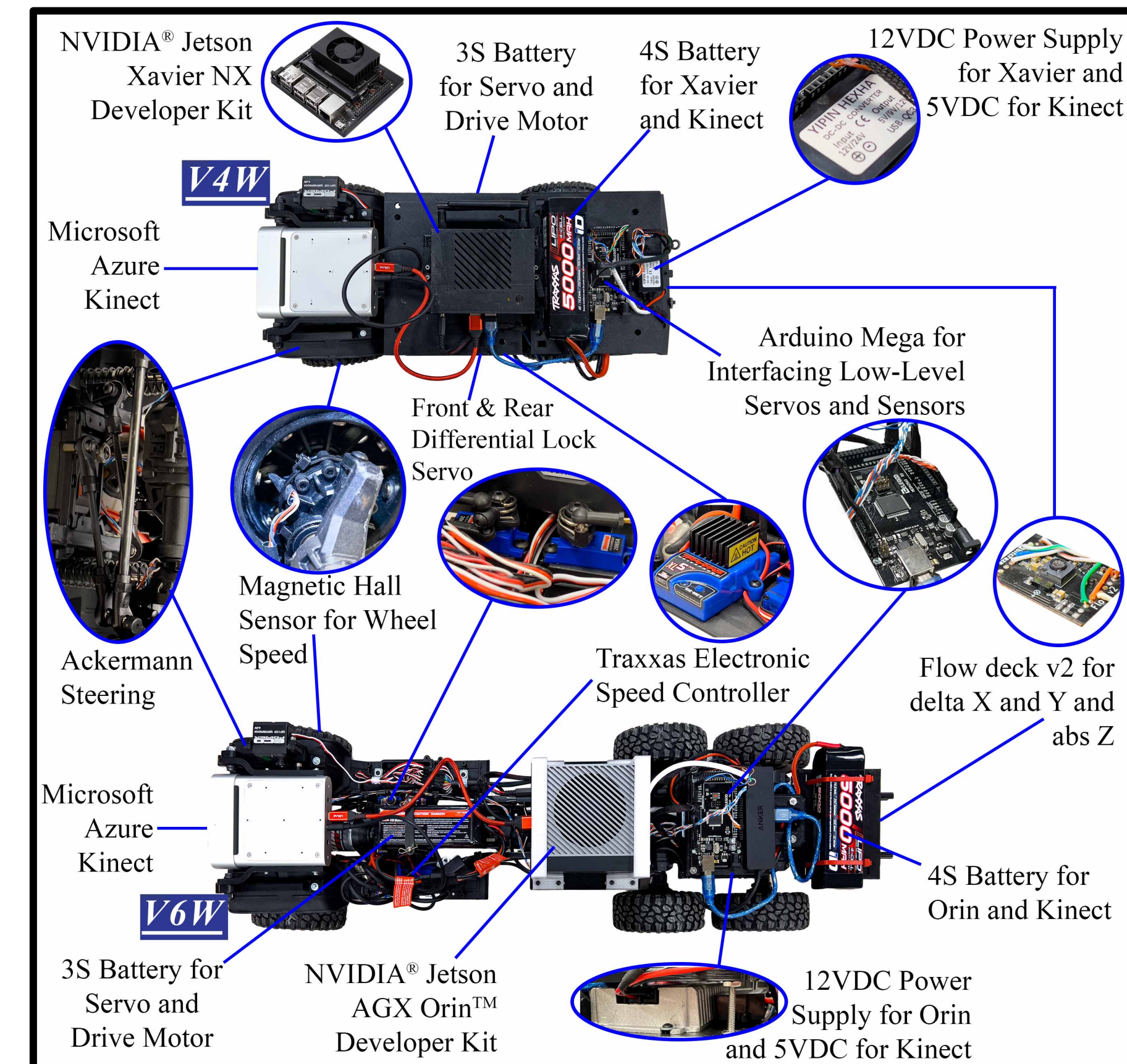
Verti-Wheelers Platforms
