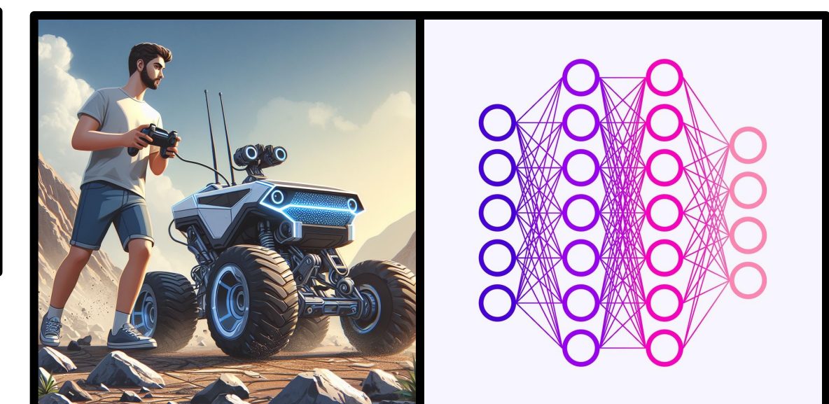
Behavior Cloning
