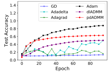
(c). kMNIST
