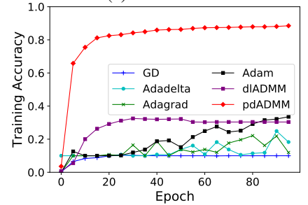
(f). CIFAR100
